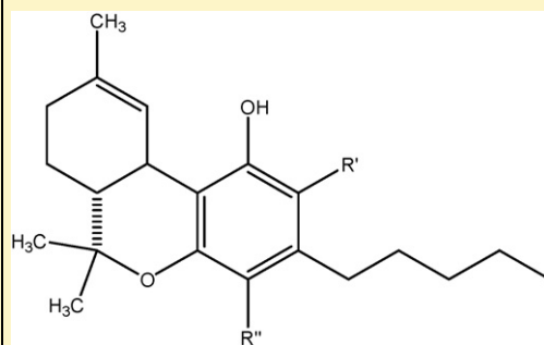
\Delta^9 -tetrahydrocannabinolic acid ( \Delta^9 -THCA)
